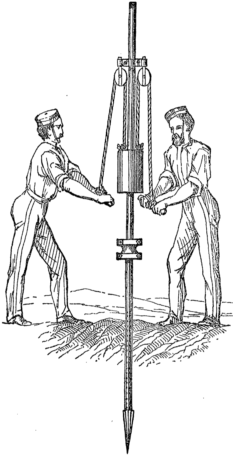
American Tube Well.
